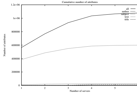
Figure 4: Cumulative number of attributes in n servers
